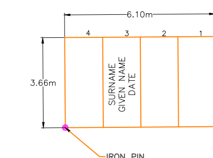
TYPICAL PLOT BLOCK B, C, D N.T.S.
